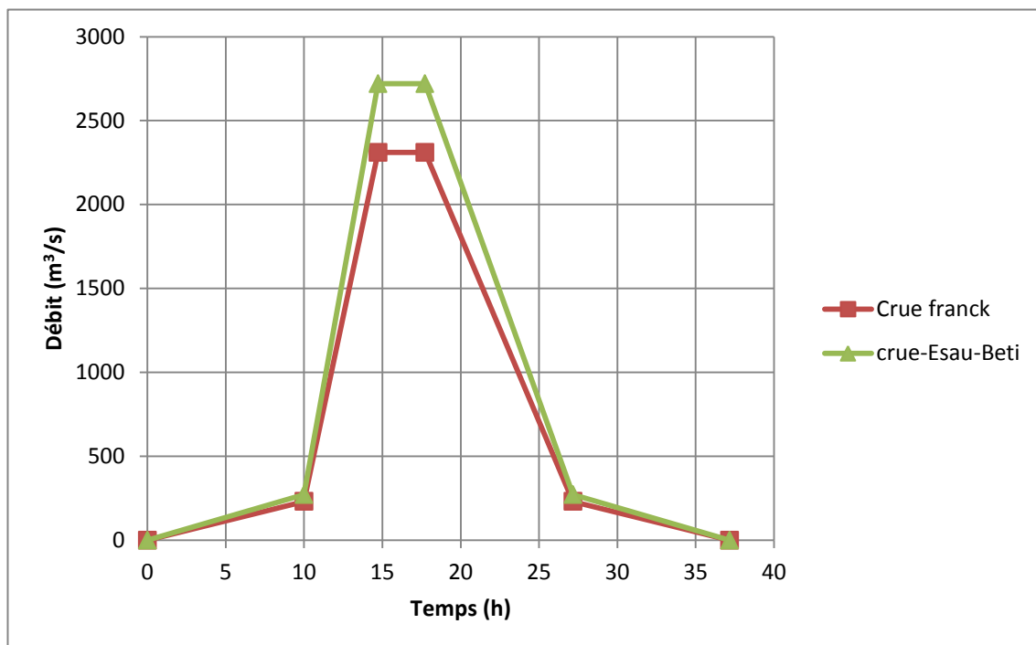
Hydrogramme – H1
