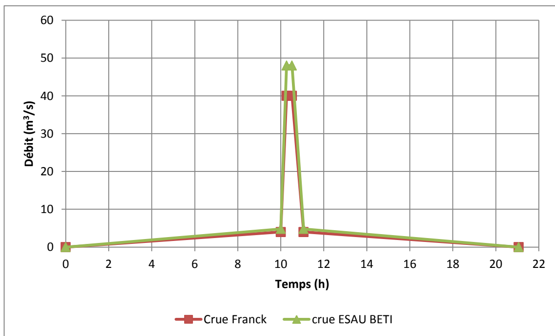
Hydrogramme – H1
