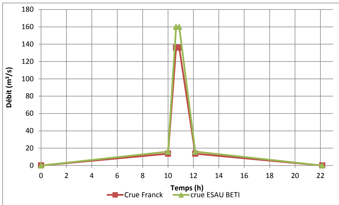
Hydrogramme – H3 – Nindia
