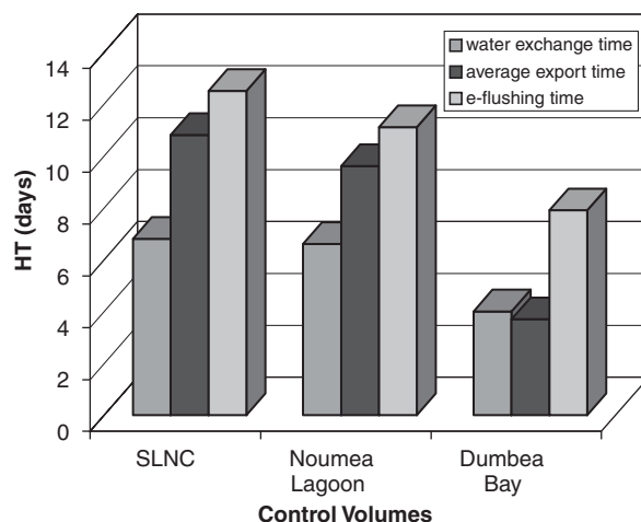
Fig. 12. General hydrodynamic time scales calculated for three different control volumes.
