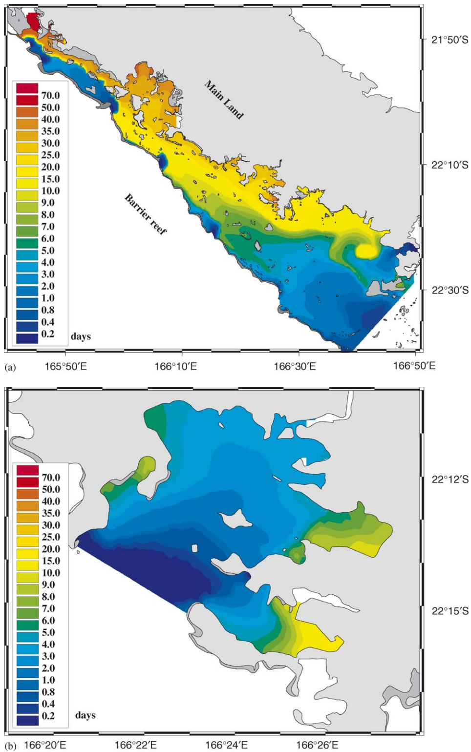
Fig. 8. Flushing lag distribution for two control volumes: (a) the SLNC, (b) the Dumbea Bay.
