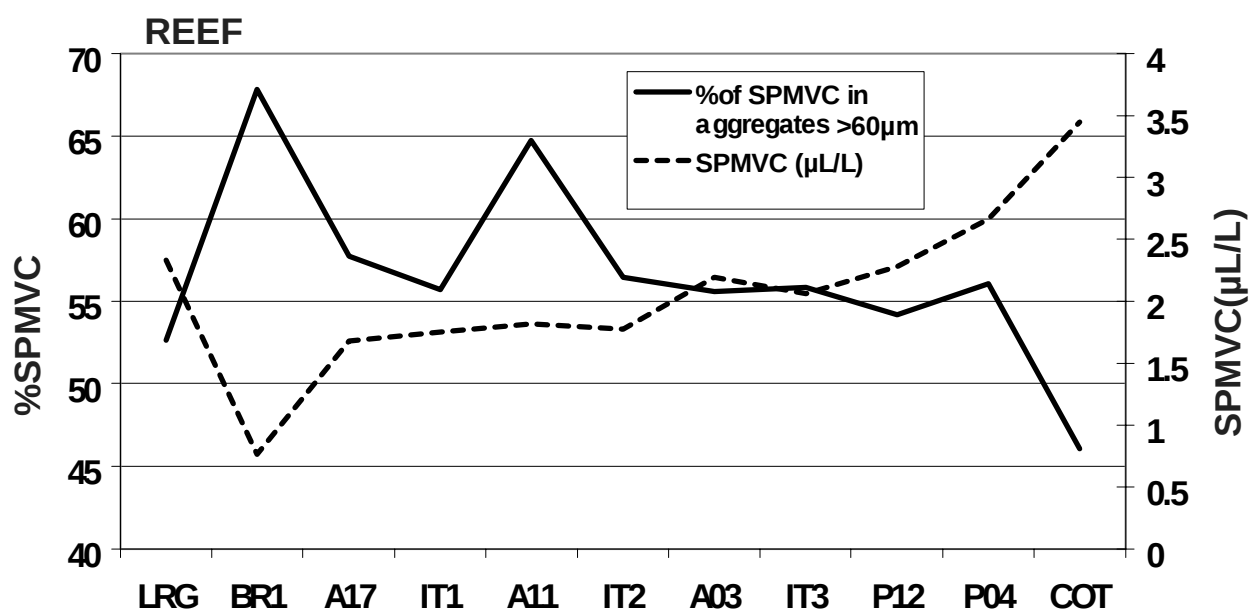
Figure 11 SPMVC and Percentage of SPM volume concentration in aggregates of diameter > 60µm along a coast-large transect.
