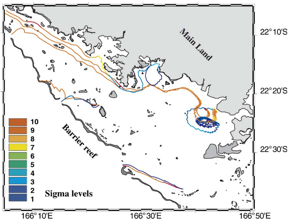
Fig. 4. Example of Lagrangian particle trajectories under forcing conditions: tide and trade winds ( 110^\circ , 8 \text{ m s}^{-1} ).
