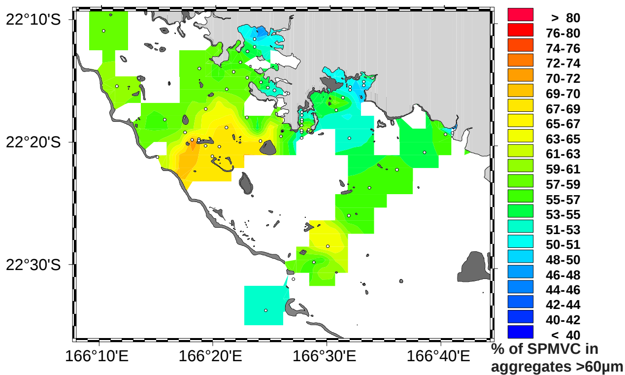
Figure 10 Percentage of SPM volume concentration in aggregates of diameter > 60µm.
