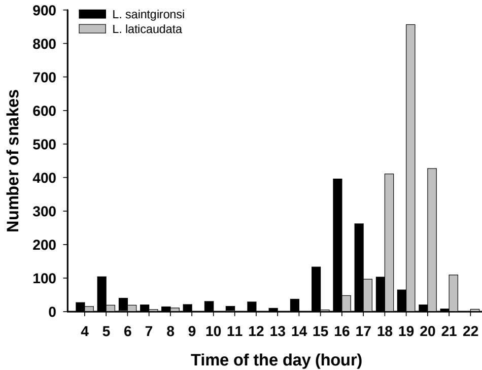
FIG. 6 - Comparative pattern of catchability of L. saintgironi (black bars) versus L. laticaudata (grey bars). Each bar represents the total number of snakes observed per-hour.
