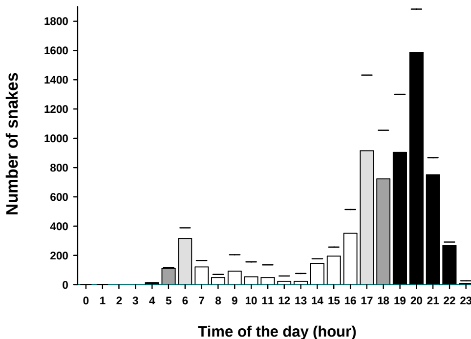
FIG. 1 - Pattern of catchability of two species of sea snakes ( L. saintgironi & L. laticaudata ) on Signal Island, New Caledonia. Each bar represents the total number of snakes counted per-hour. The grey-black colouration provides a rough scale for sunlight, from full day (white), partial darkness (grey) to full darkness (black). The line above each bar indicates the value when data from 8 other islets (see text) have been added.
