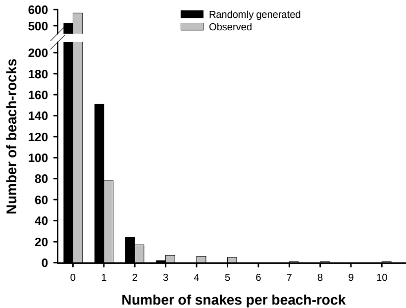
FIG. 8 - Distribution of the number of snakes found under each lifted beach-rocks. The randomly generated distribution is the mean of 200 random distribution. Theoretically, 3 snakes under one beach-rocks is the maximum value. The observed distribution show that up to 10 snakes can co-occur under a single beach-rock.
